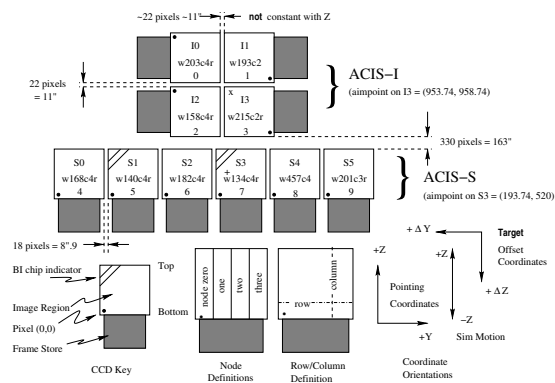
Figure 4.6: The Layout of ACIS (Chandra X-ray Center, 2022).
