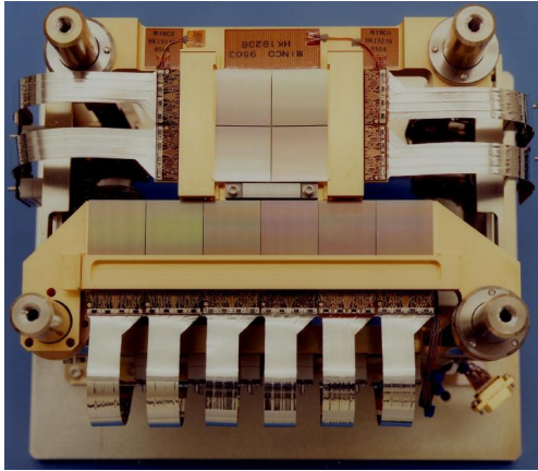
Figure 4.6: The Layout of ACIS (Chandra X-ray Center, 2022).
