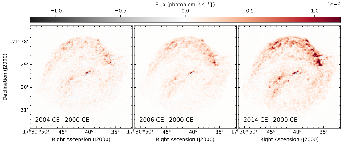
Figure 6.7: The images of flux change of Kepler’s SNR in the energy band of 0.5–0.7 keV. The images are made by subtracting Chandra flux images taken in 2000 from 2004 (left), 2006 (middle), and 2014 (right). The positive values represent the brightening.
